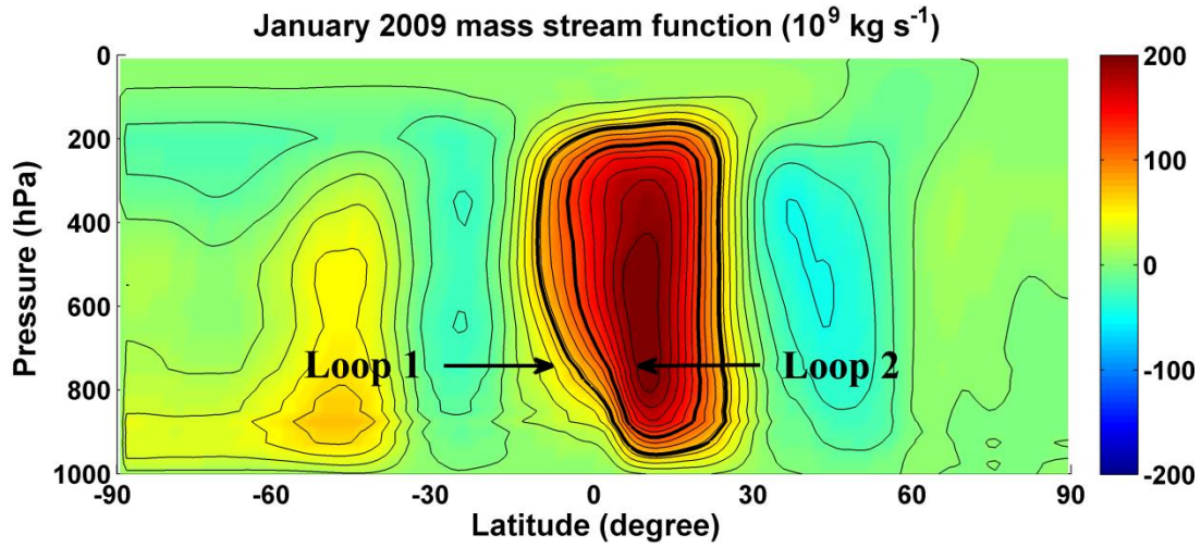
Fig.S1: Schematic illustration of the method used in quantifying the power of Hadley cells.
